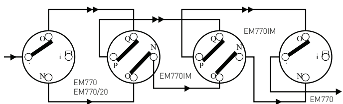
MULTIWAY SWITCHING MORE THAN 2 SWITCHES (Any quantity of intermediate switches may be used).
